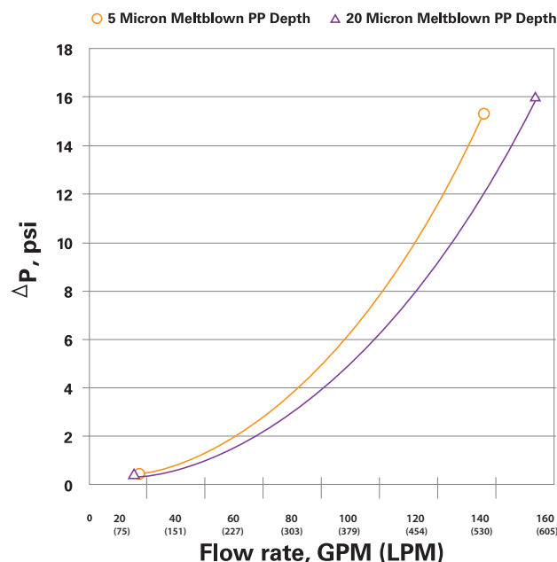
Filter Performance
