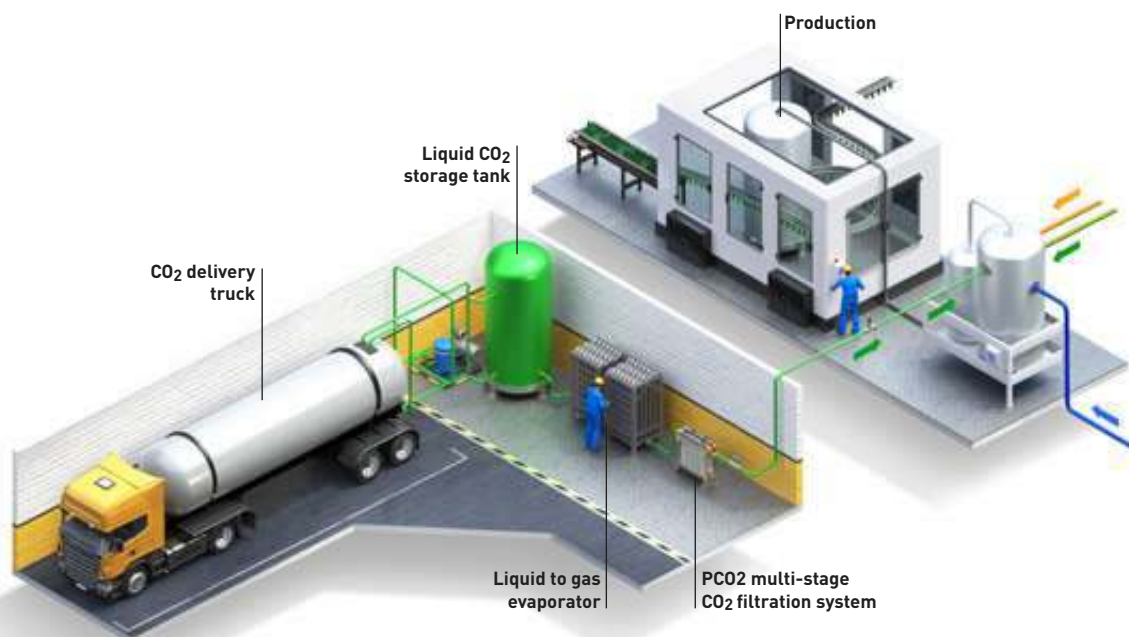
Typical production plant application
