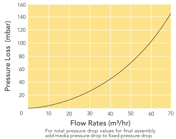
Fixed Pressure Drop Values for HFC Hardware
